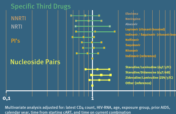
Figure 3 Rate ratios of AIDS/death (95% CI) comparing different nucleoside pairs and specific third drugs
